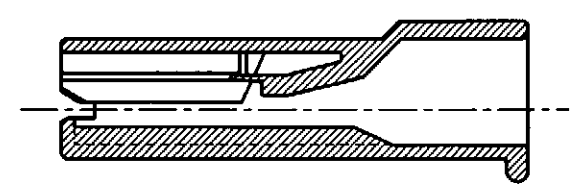
断面 "A" - "A" SECT.
