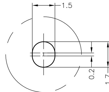
DETAIL F SCALE 8:1
