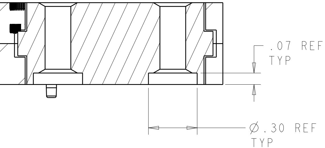
SECTION B-B ROTATED 90° CW
