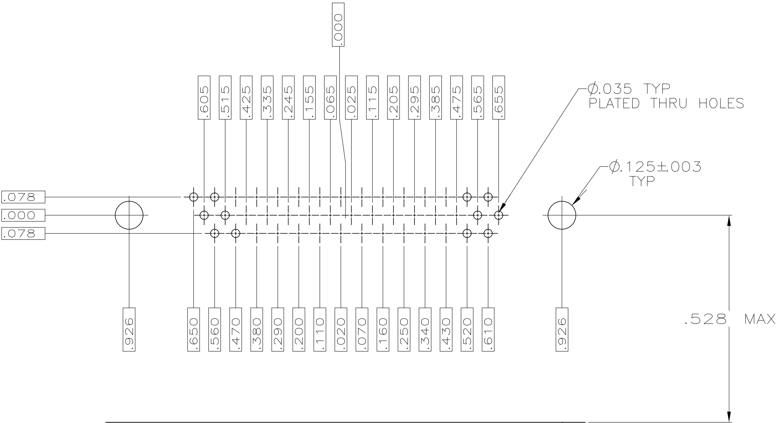
SHELL SIZE 3 (44 POSITION)
