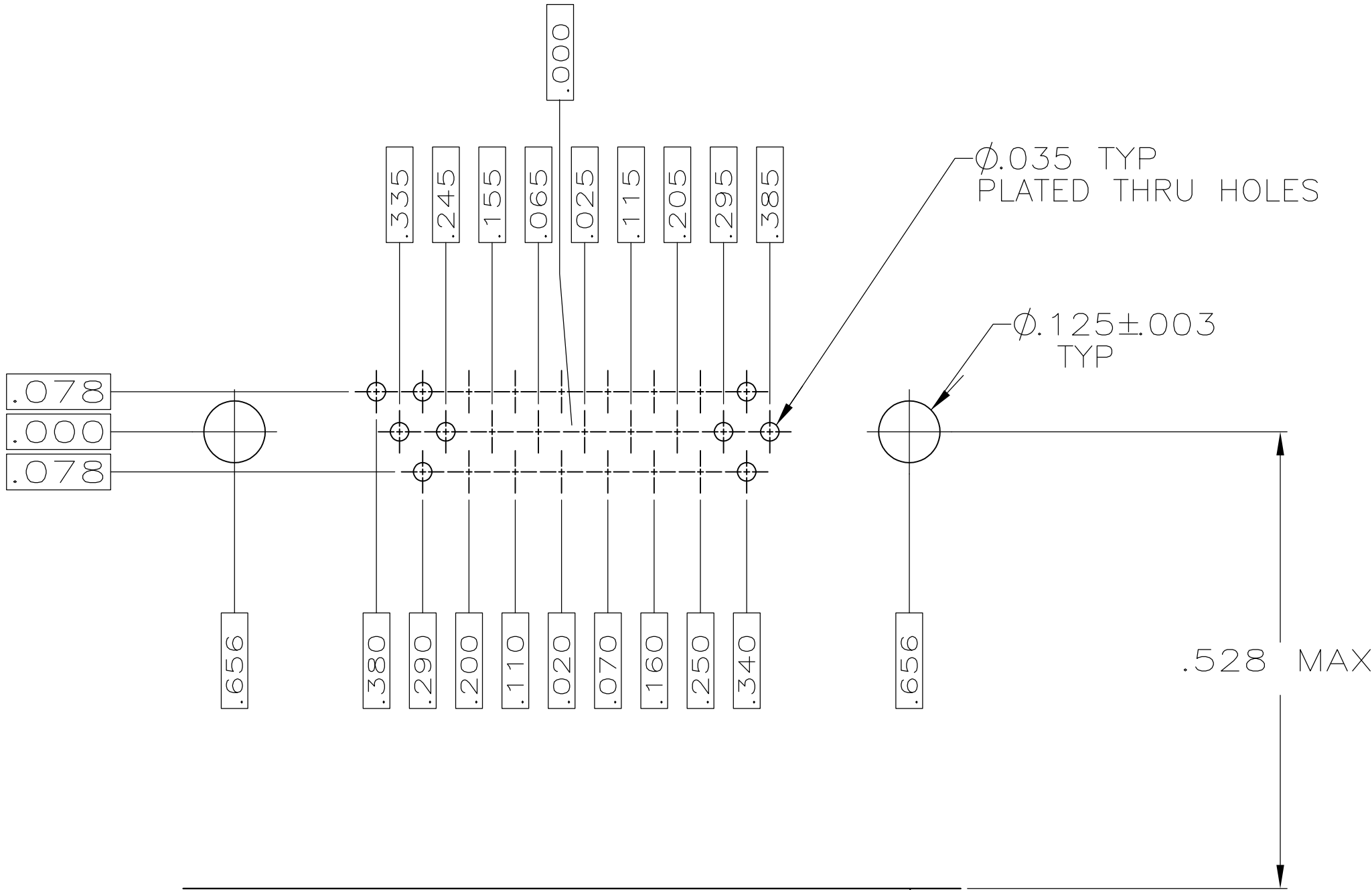
SHELL SIZE 2 (26 POSITION)
