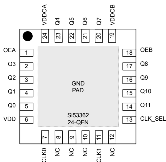
Figure 5.3. Si53362 Pin Descriptions
