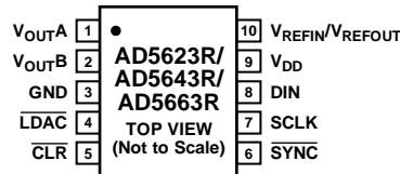
Figure 3. Pin Configuration
