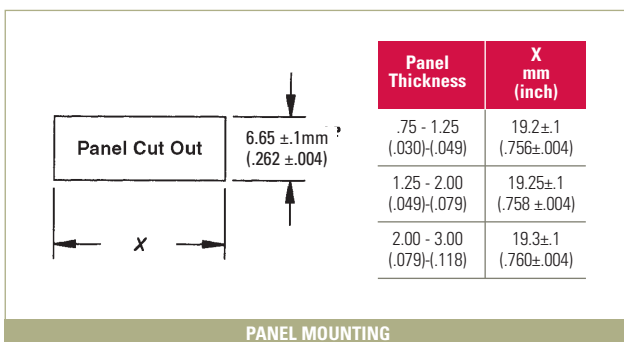
PANEL MOUNTING
