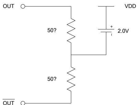
LVPECL Levels Test Circuit
