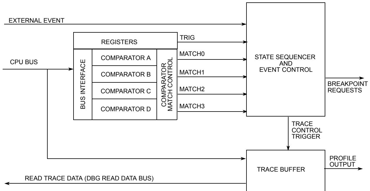
Figure 67. Debug module block diagram
