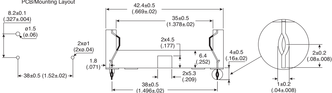
PCB/Mounting Layout
