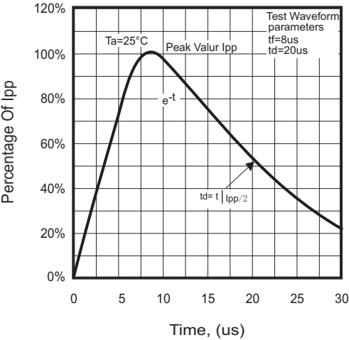
Fig.1 - Peak Pulse Current Wave Form Acc. IEC 61000-4-5
