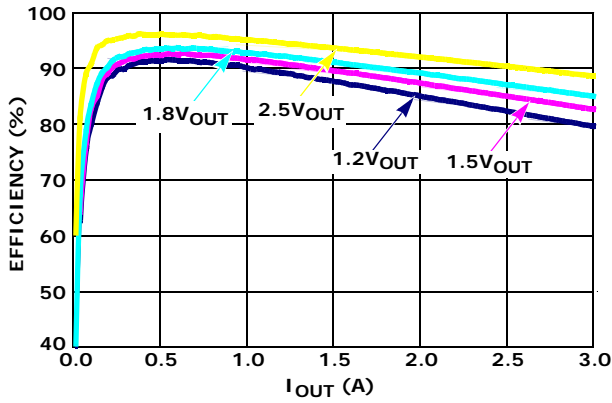
FIGURE 3. EFFICIENCY, T_A = +25^\circ\text{C} , V_{IN} = 3.3\text{V}
