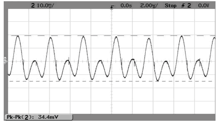
Output Ripple and Noise (Vin=5V, Vout=1.8V, Iout=3A, Cloud=0, ScopeBW=100MHz)
