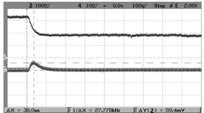
Step Load Transient Response (Vin=5V, Vout=1.8V, Cloud=0, Iout=3A to 1.5A) Trace 2=Vout, 100 mV/div. Trace 4=Iout, 1A/div.
