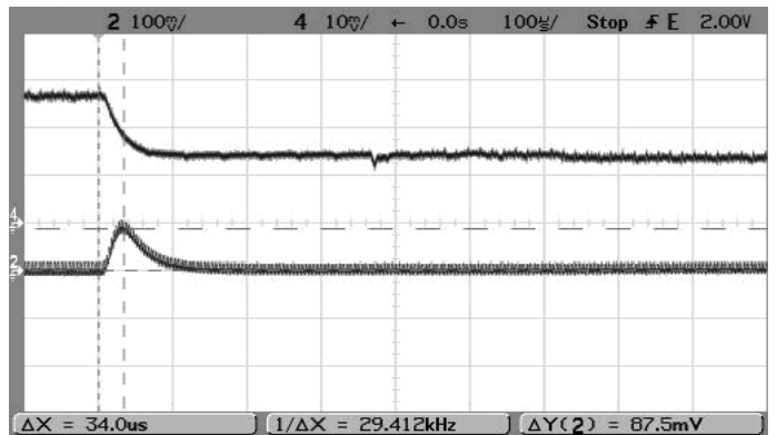
Step Load Transient Response (Vin=5V, Vout=1.8V, Cload=0, Iout=5A to 2.5A) Trace 2=Vout, 100 mV/div. Trace 4=Iout, 2A/div.
