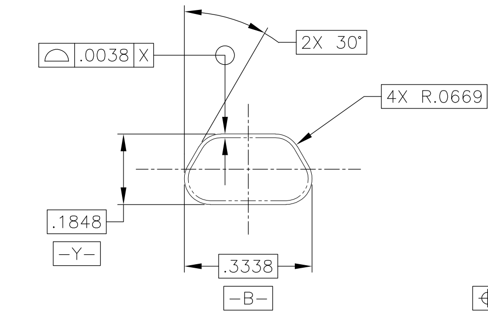
INTERFACE DETAIL
