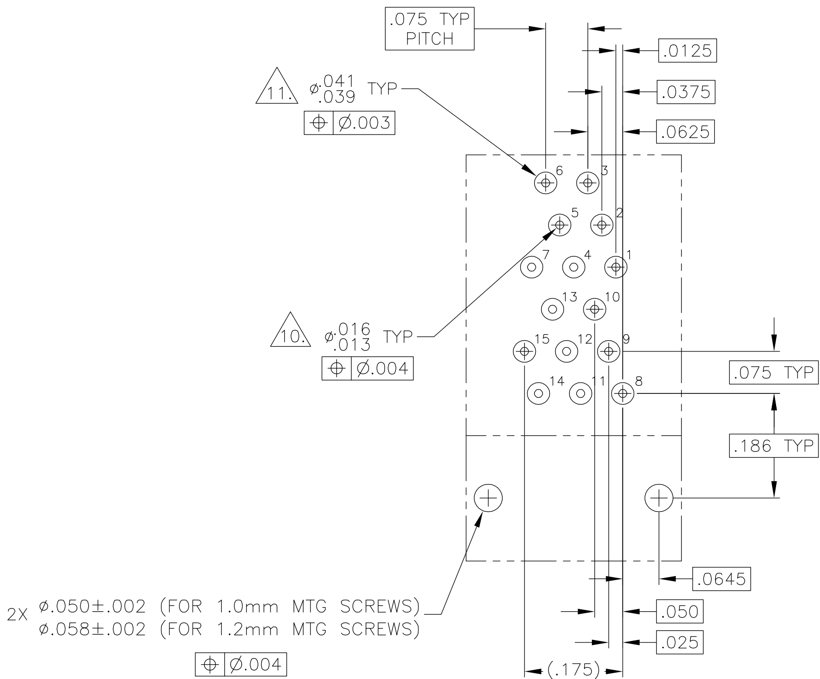
TYPICAL PCB LAYOUT SIZE 15 SHOWN FOR REFERENCE
