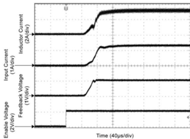
Start-Up Waveforms
