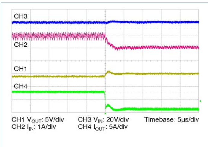
Figure 16 — 7.3A - 0A transient response. C_{IN} = 100µF, no external C_{OUT}
