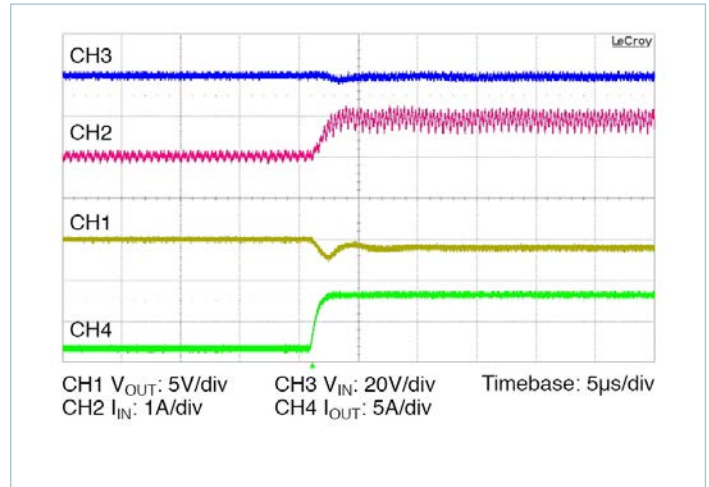
Figure 15 — 0A - 7.3A transient response. C_{IN} = 100µF, no external C_{OUT}
