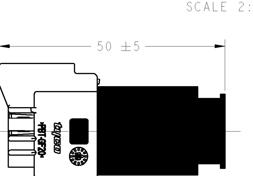
NECESSARY VOLUME FOR ASSEMBLY ON THE TAB HOUSING
