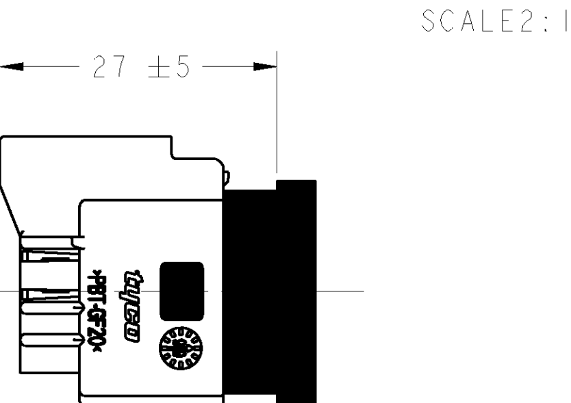
NECESSARY VOLUME FOR ASSEMBLY HEADER
