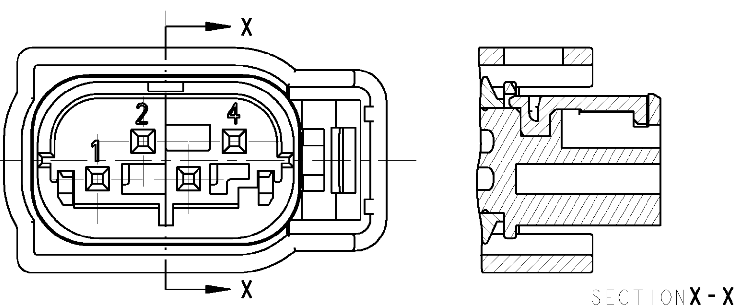
POSITION OF ASSEMBLY locking device locking
