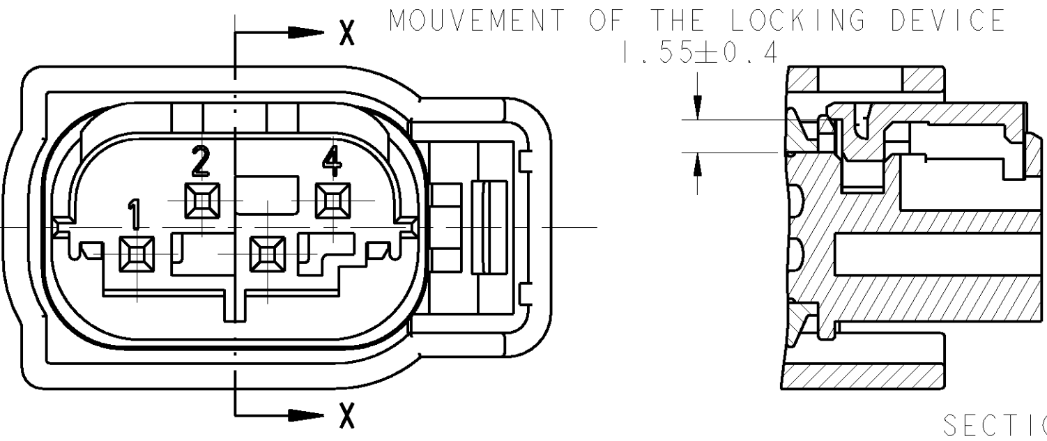
POSITION OF DELEVERY locking device in position pre-locked
