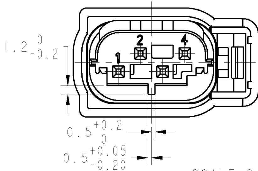
REF TE 1379799-2 CODING B
