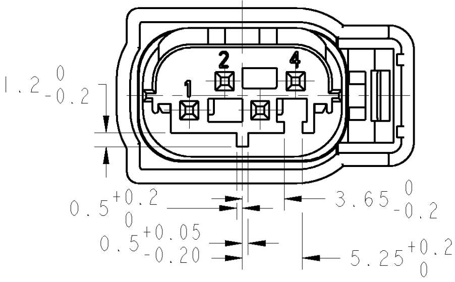
REF TE 1379799-2 CODING B
