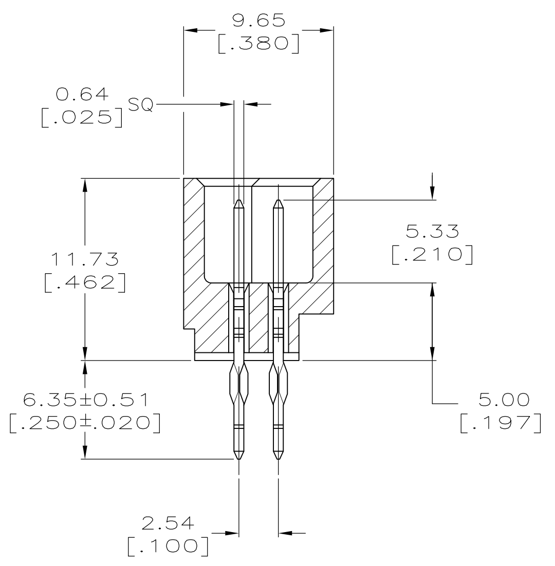
SECTION T-T
