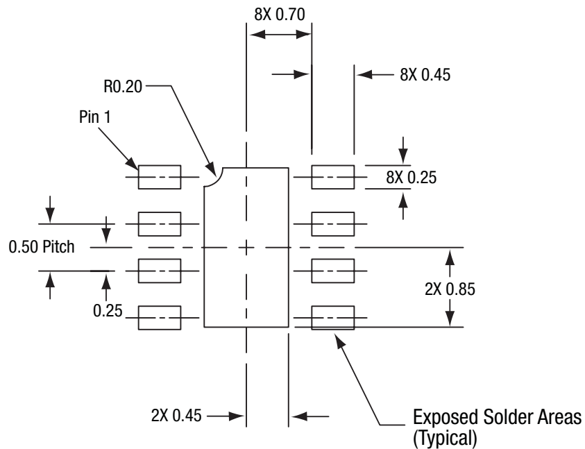
Figure 33. SKY65048-360LF PCB Layout Footprint
