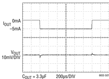
1.25V Sourcing Current with a 3.3μF Output Capacitor
