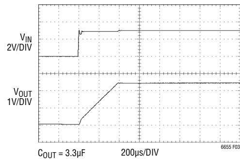
Figure 3. Start-Up Response
