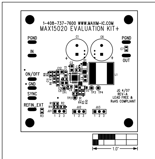
Figure 2. MAX15020 EV Kit Component Placement Guide—Component Side
