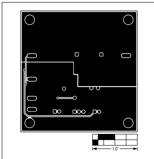
Figure 4. MAX15020 EV Kit PCB Layout—GND Layer 2
