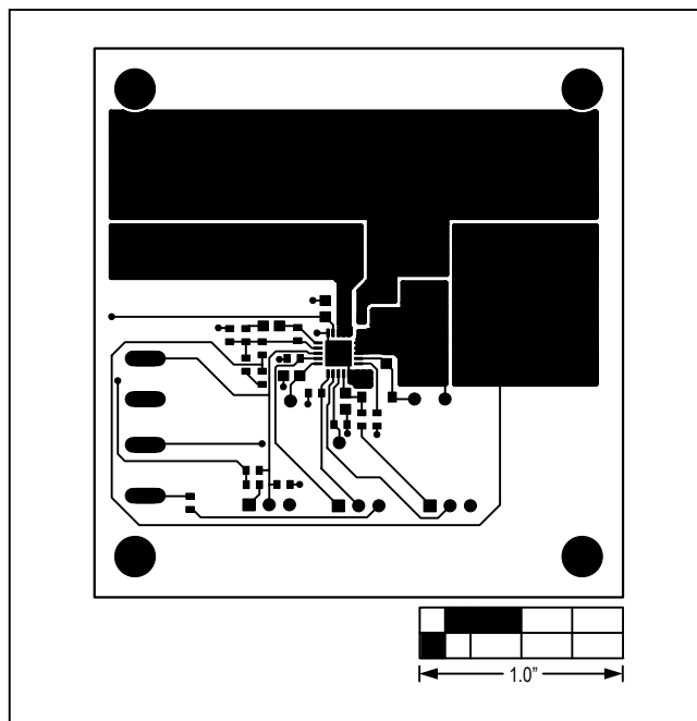
Figure 3. MAX15020 EV Kit PCB Layout—Component Side
