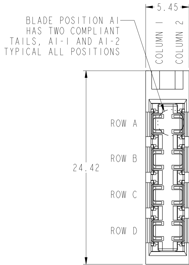
1-SLOT POWER MODULE MATING-FACE VIEW SCALE 4:1
