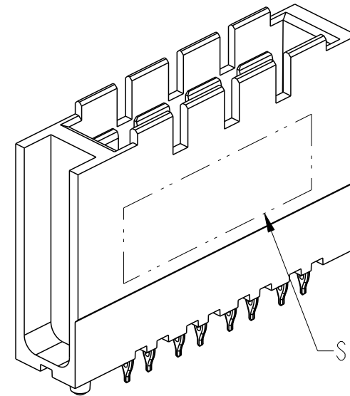
ISOMETRIC VIEW 1 POSITION
