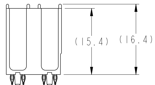
2-SLOT POWER MODULE BACK VIEW
