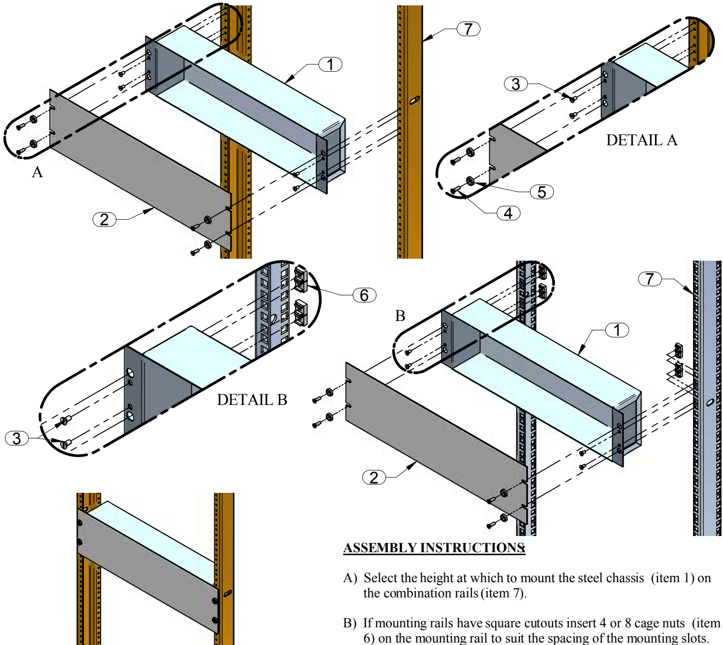
COMPLETE ASSEMBLY
