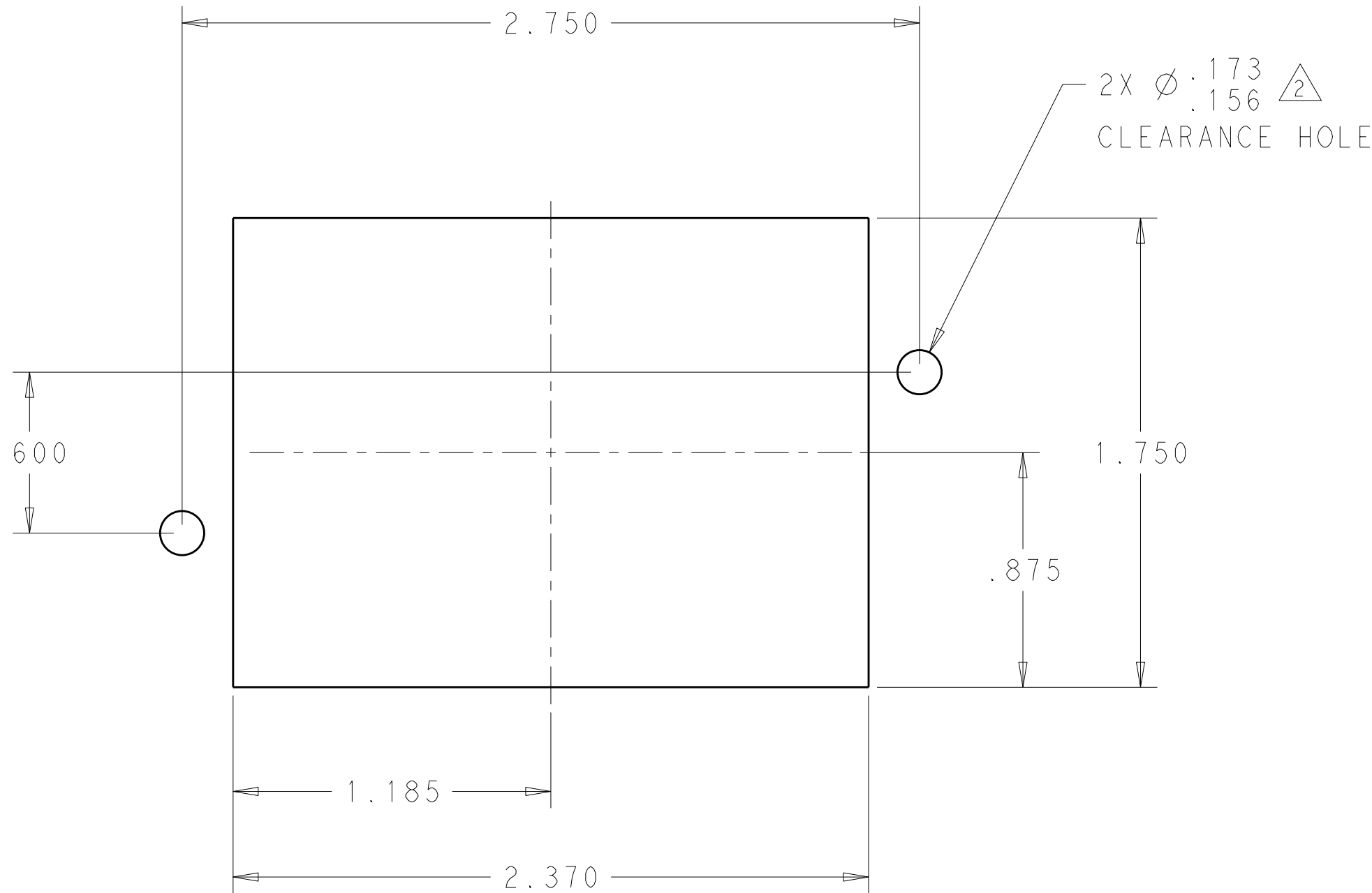
PIN CONNECTOR PANEL CUT-OUT
