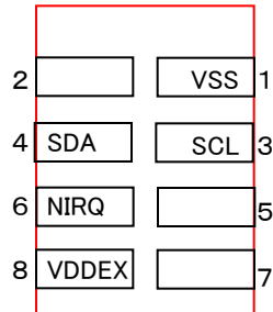
DF11CZ-8DP-2V(27) ( Hirose Electric )
