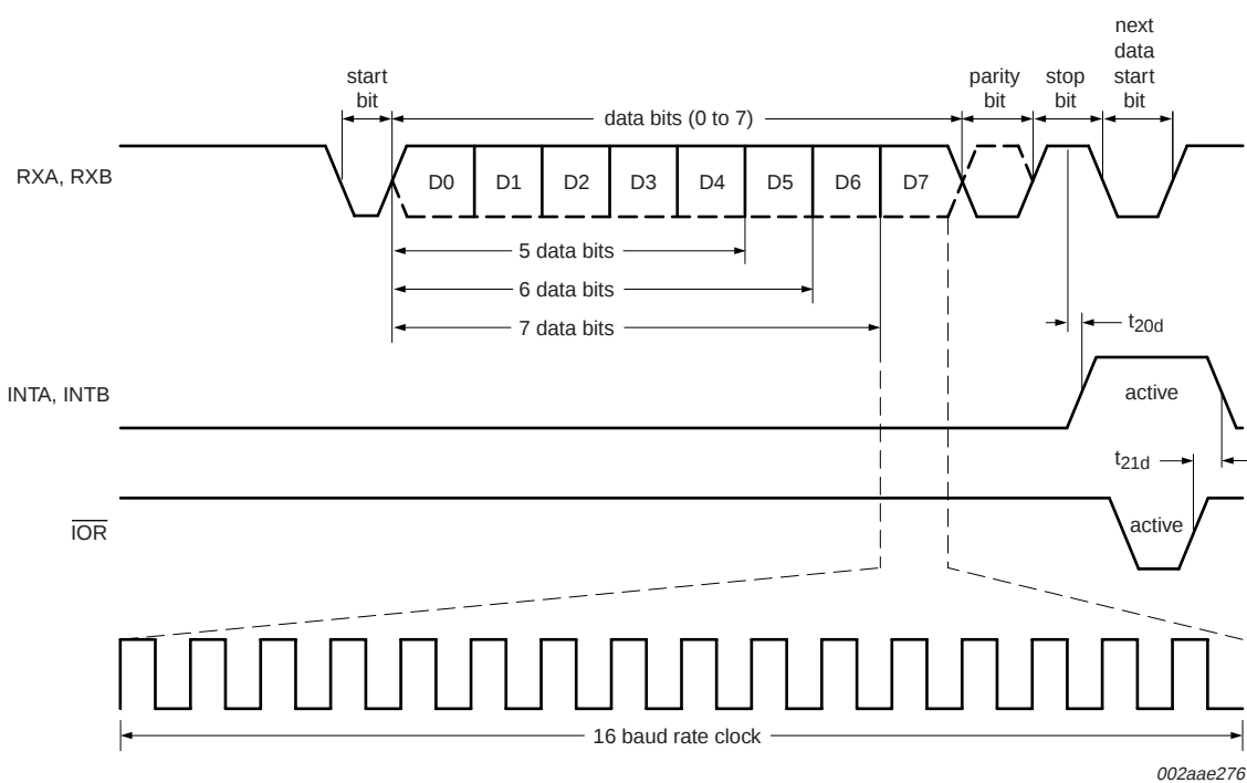
Fig 12. Receive timing
