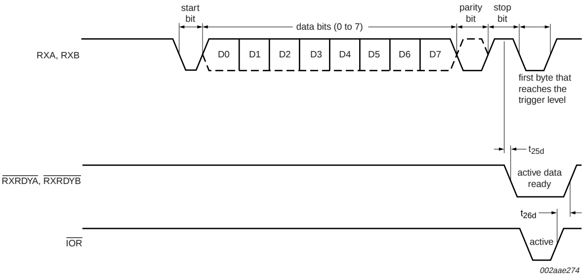
Fig 14. Receive ready timing in FIFO mode
