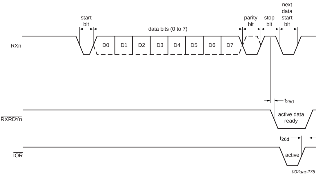
Fig 13. Receive ready timing in non-FIFO mode
