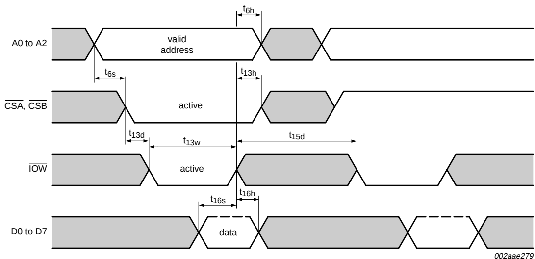
Fig 8. General write timing
