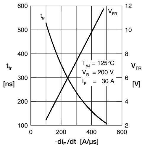
Fig. 6 Typ. forward recov. voltage V_{FR} V_{FR} & time t_{fr} versus di_F/dt
