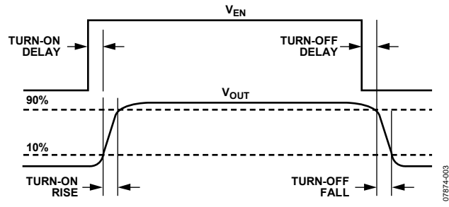
Figure 3. Timing Diagram
