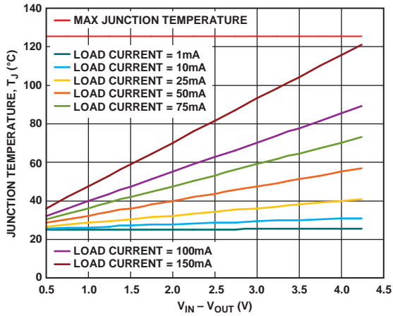
Figure 30. 500 mm 2 of PCB Copper, T A = 25°C
