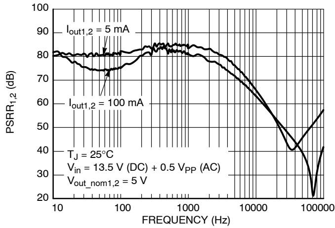
Figure 17. PSRR vs. Frequency
