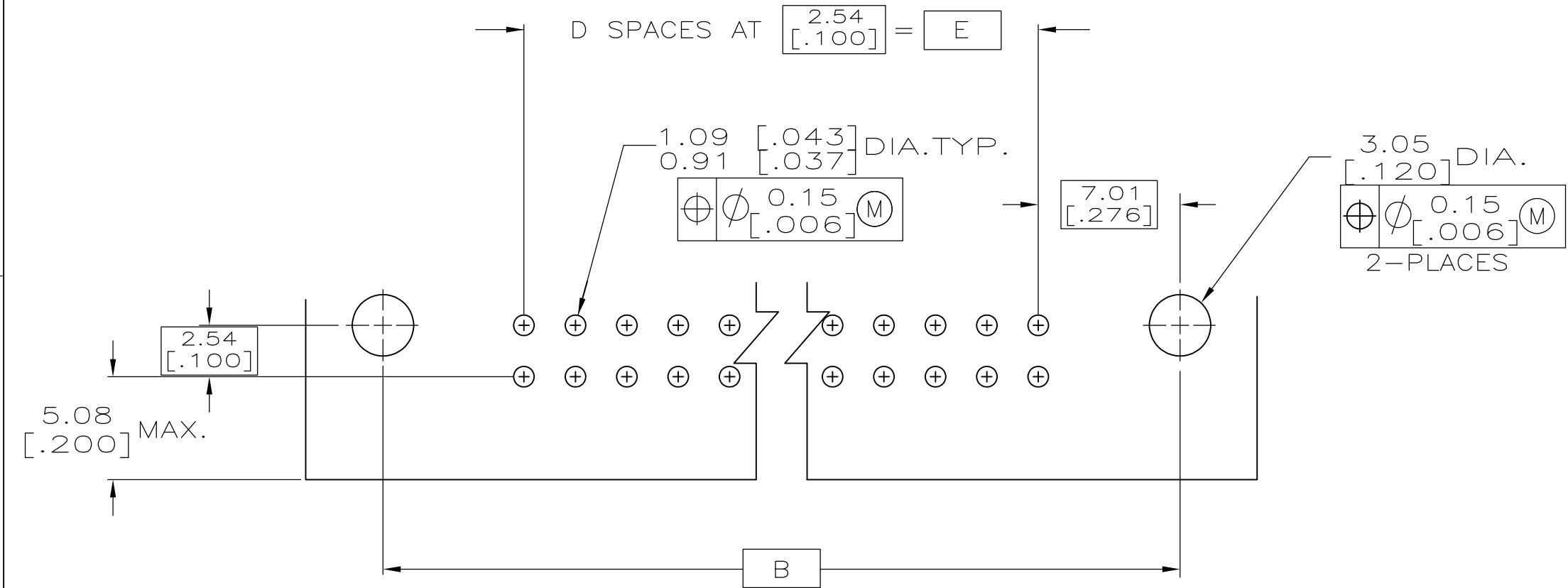
RECOMMENDED PC BOARD LAYOUT 4
