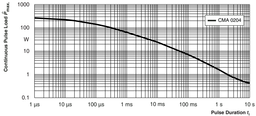
Maximum pulse load, continuous pulse; applicable if \bar{P} \leq P(\vartheta_{amb}) and \hat{U} \leq 2 \text{ kV} ; for permissible resistance change \pm (0.5 \% R + 0.05 \Omega)
