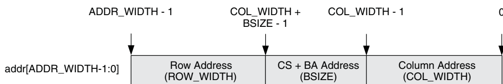
Figure 2-6. Local-to-Memory Address Mapping for Memory Access
