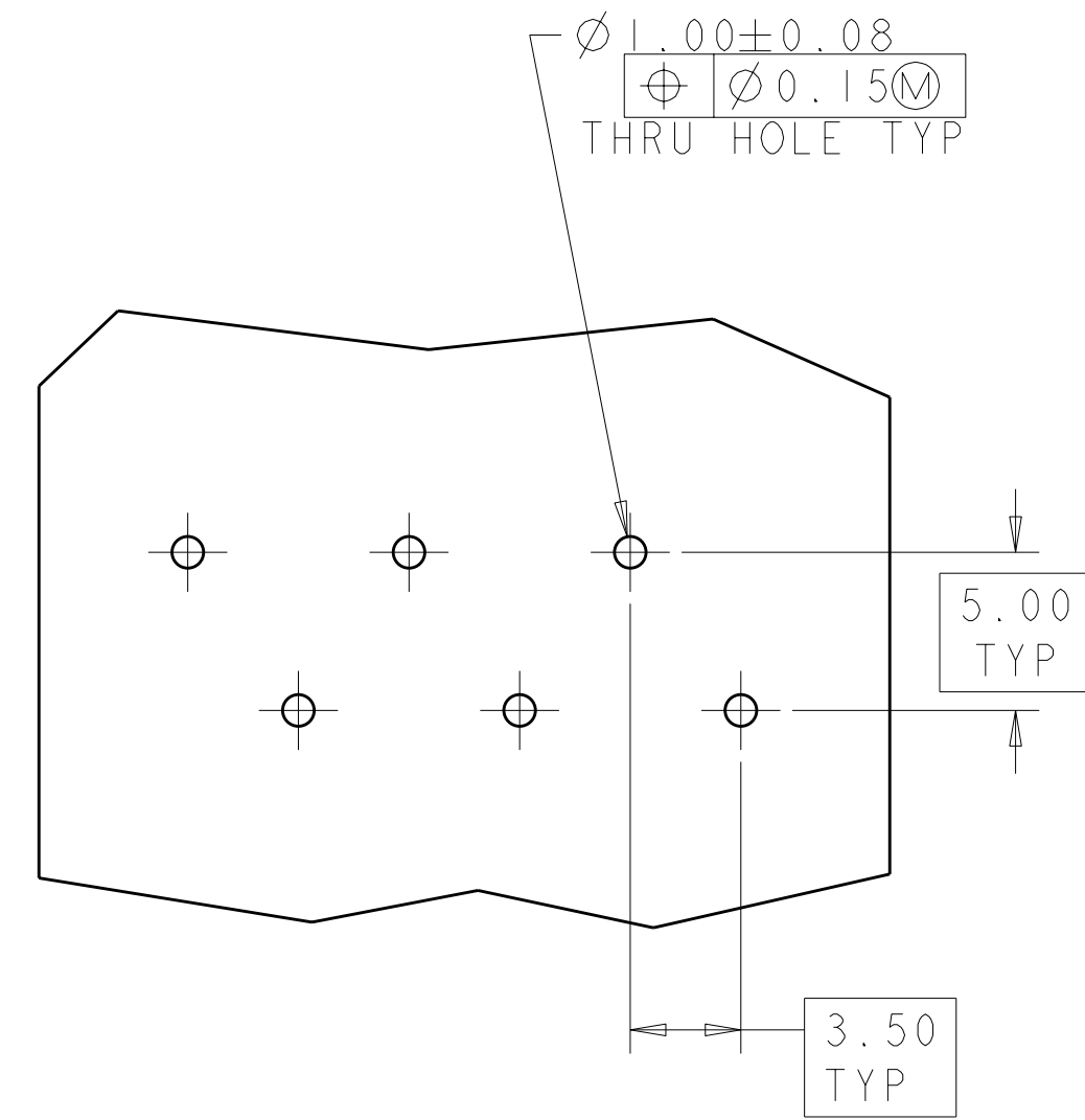
5 PCB FOOTPRINT SCHEME B SCALE 4:1
