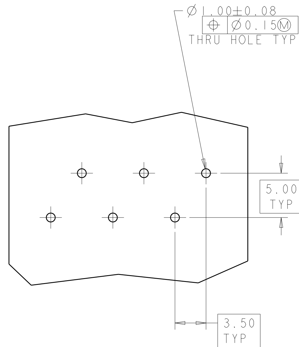
5 PCB FOOTPRINT SCHEME A SCALE 4:1
