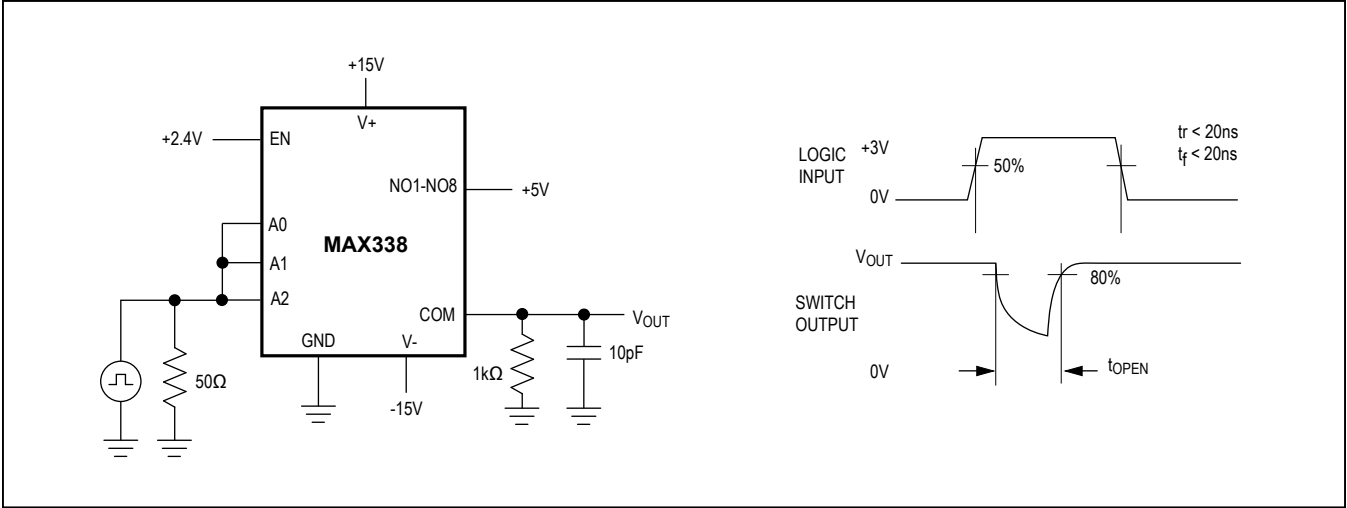
Figure 4. Break-Before-Make Interval
