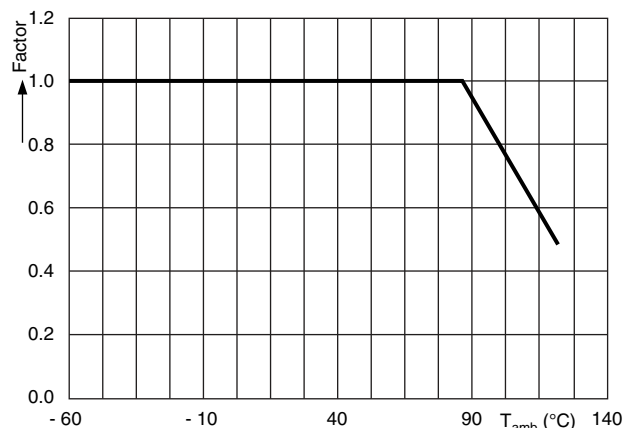
Nominal voltage (AC and DC) as a function of temperature
