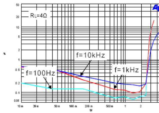
2. THD+N vs Output Power
