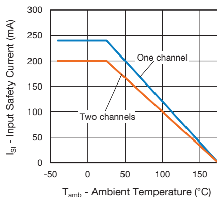
Fig. 3 - Input Safety Current vs. Ambient Temperature
