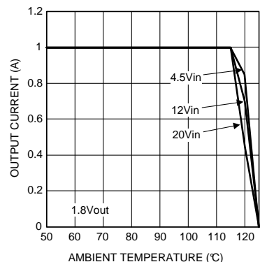
Figure 32. Thermal Derating V OUT = 1.8 V
