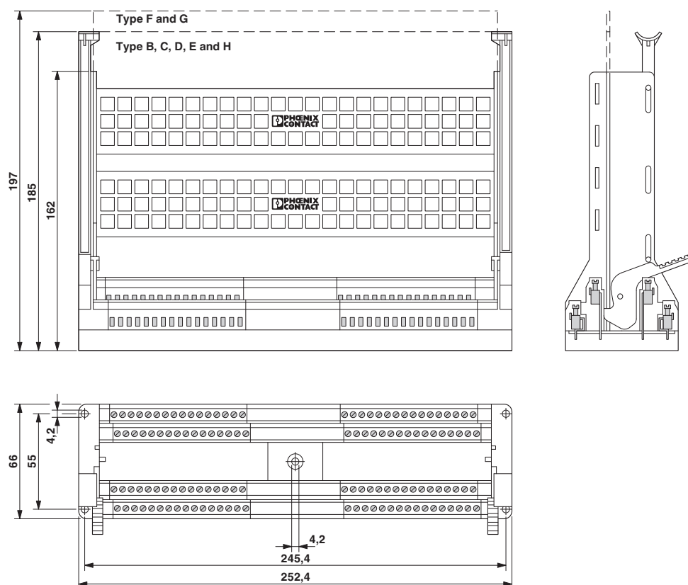
Dimensional drawing
