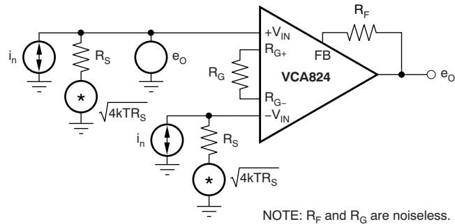
Figure 68. Simple Noise Model
