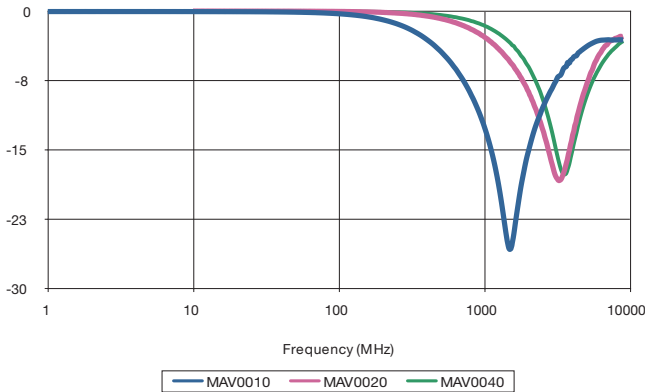
Transmission Characteristics
