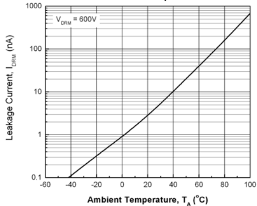
Figure 5. Leakage Current vs. Ambient Temperature
