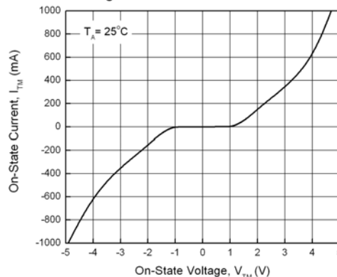
Figure 2. On-State Characteristics
