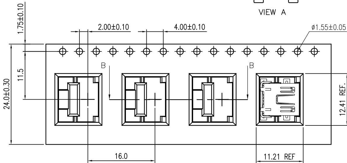
DETAIL A
