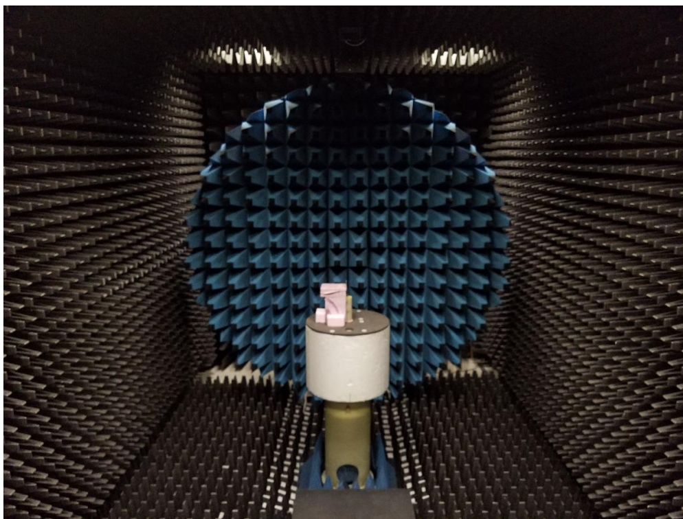
Figure 2 Antenna Chamber
