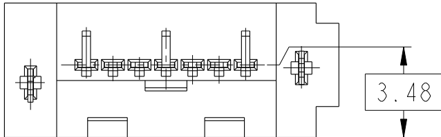
SECTION C1-C1
