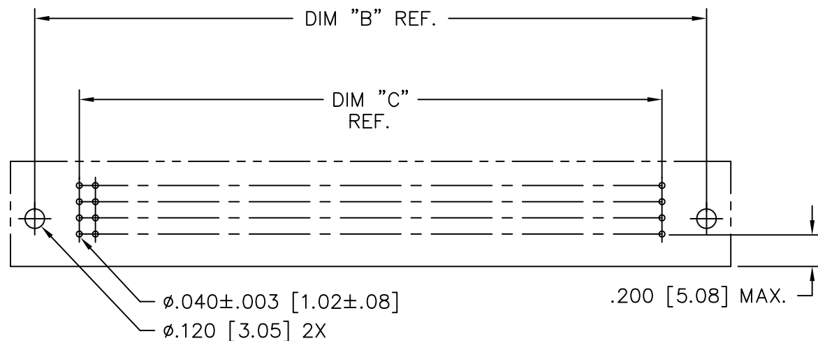
SECTION U-U
