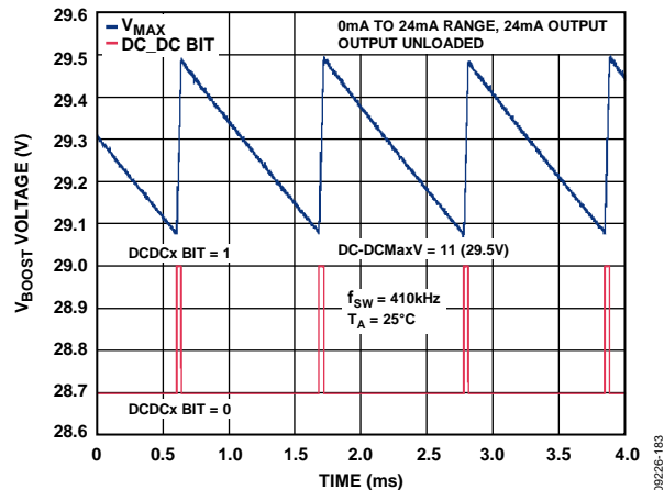
Figure 82. Operation on Reaching V MAX
