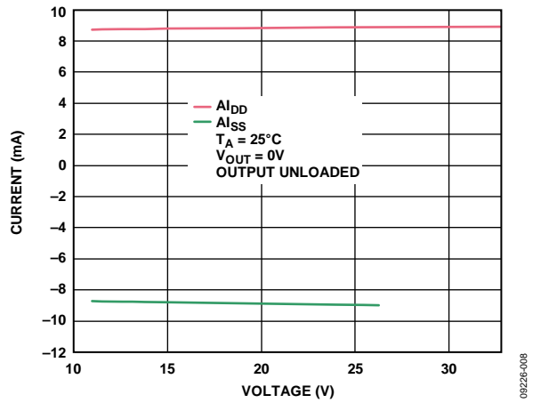
Figure 68. A I DD /A I SS vs. A V DD /A V SS
