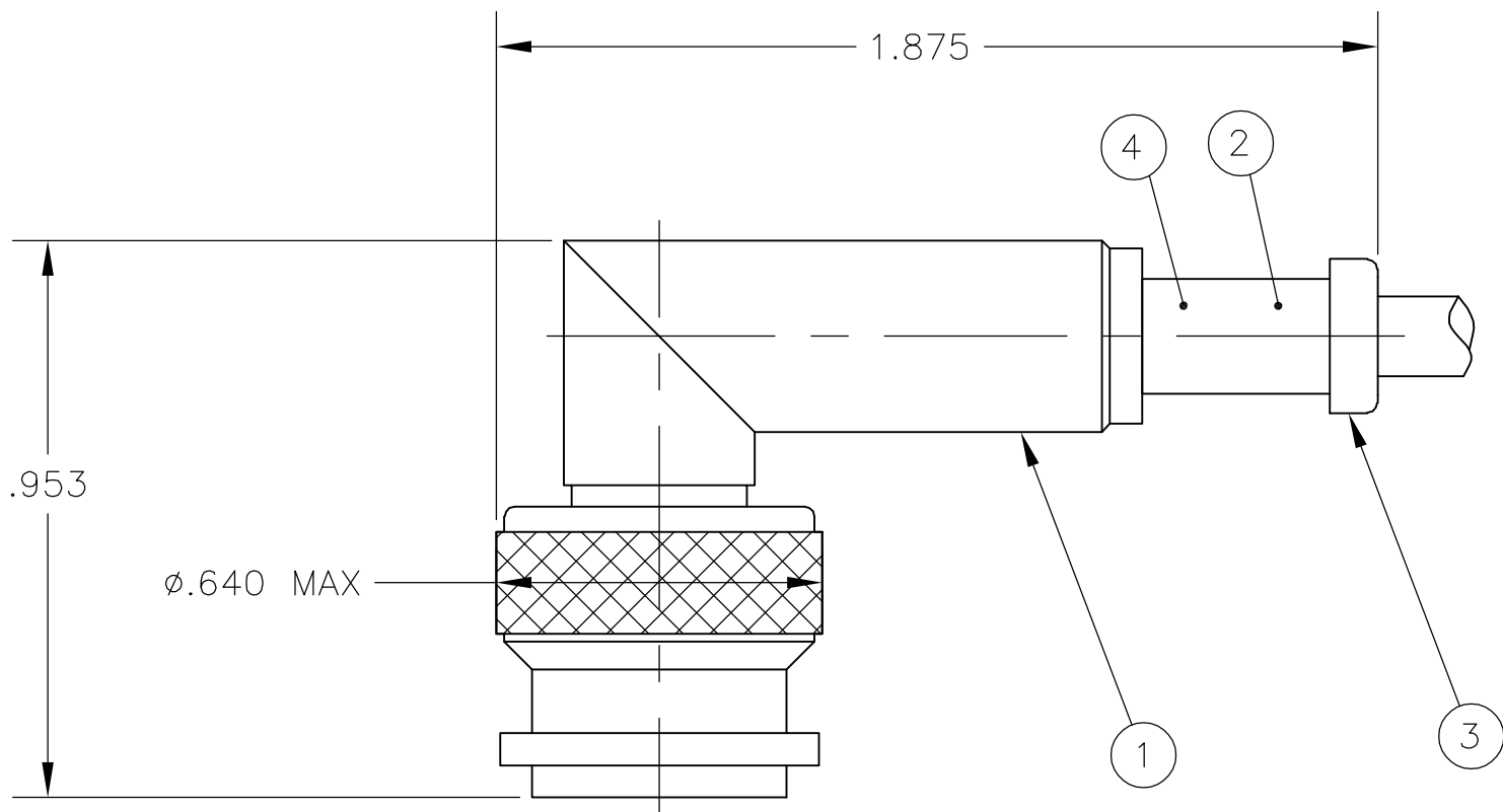
ASSEMBLED VIEW
