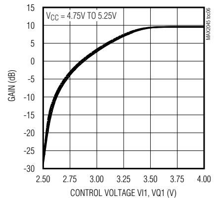
GAIN vs. CONTROL VOLTAGE (VI1 = VQ1)
