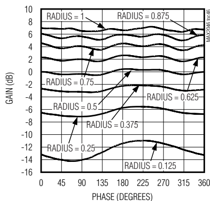
GAIN vs. PHASE
