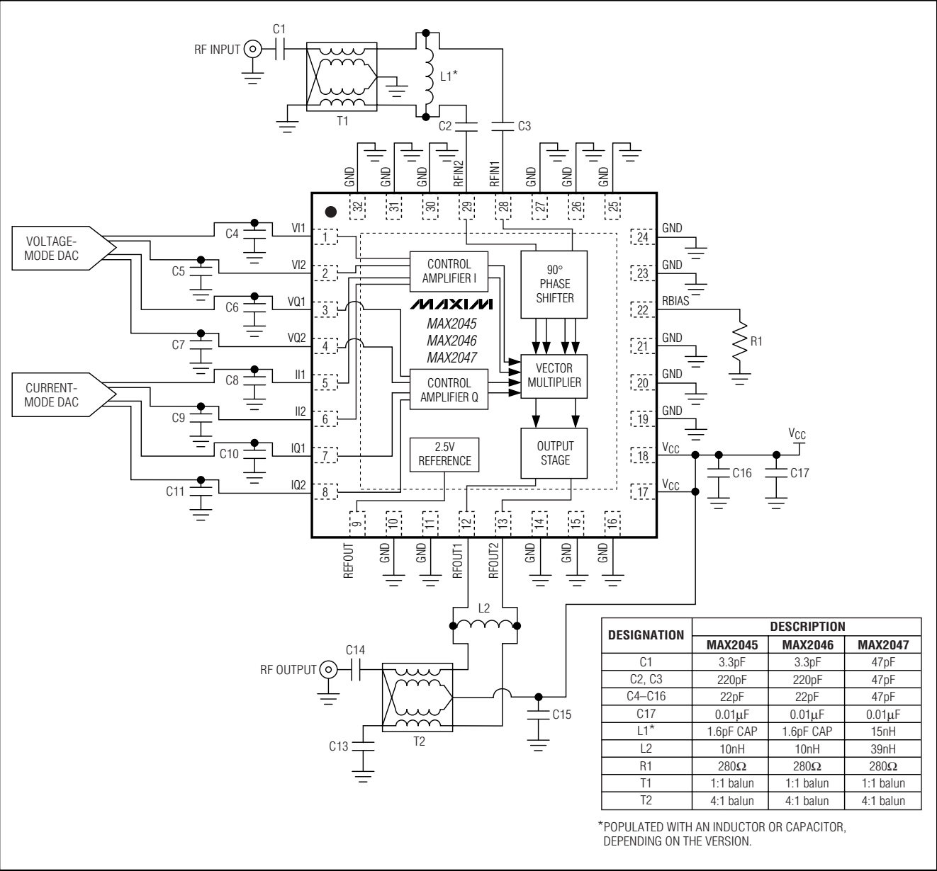
Figure 1. Typical Operating Circuit Using Differential Current- and Voltage-Mode DACs
