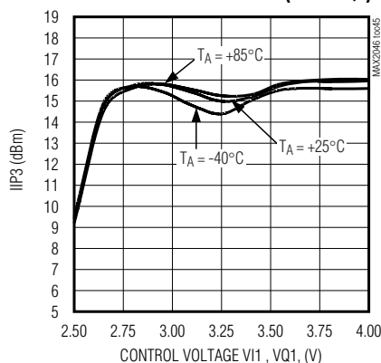
IIP3 vs. CONTROL VOLTAGE ( VI1 = VQ1 )
