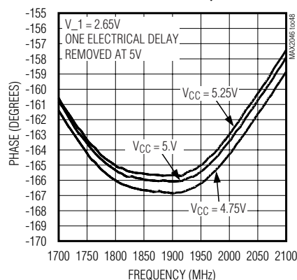
S21 PHASE vs. FREQUENCY
