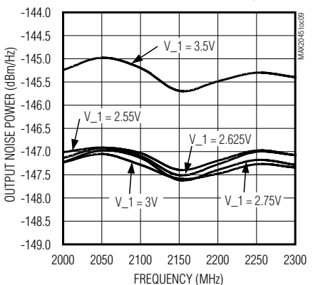
OUTPUT NOISE POWER vs. FREQUENCY
