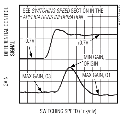
SWITCHING SPEED
