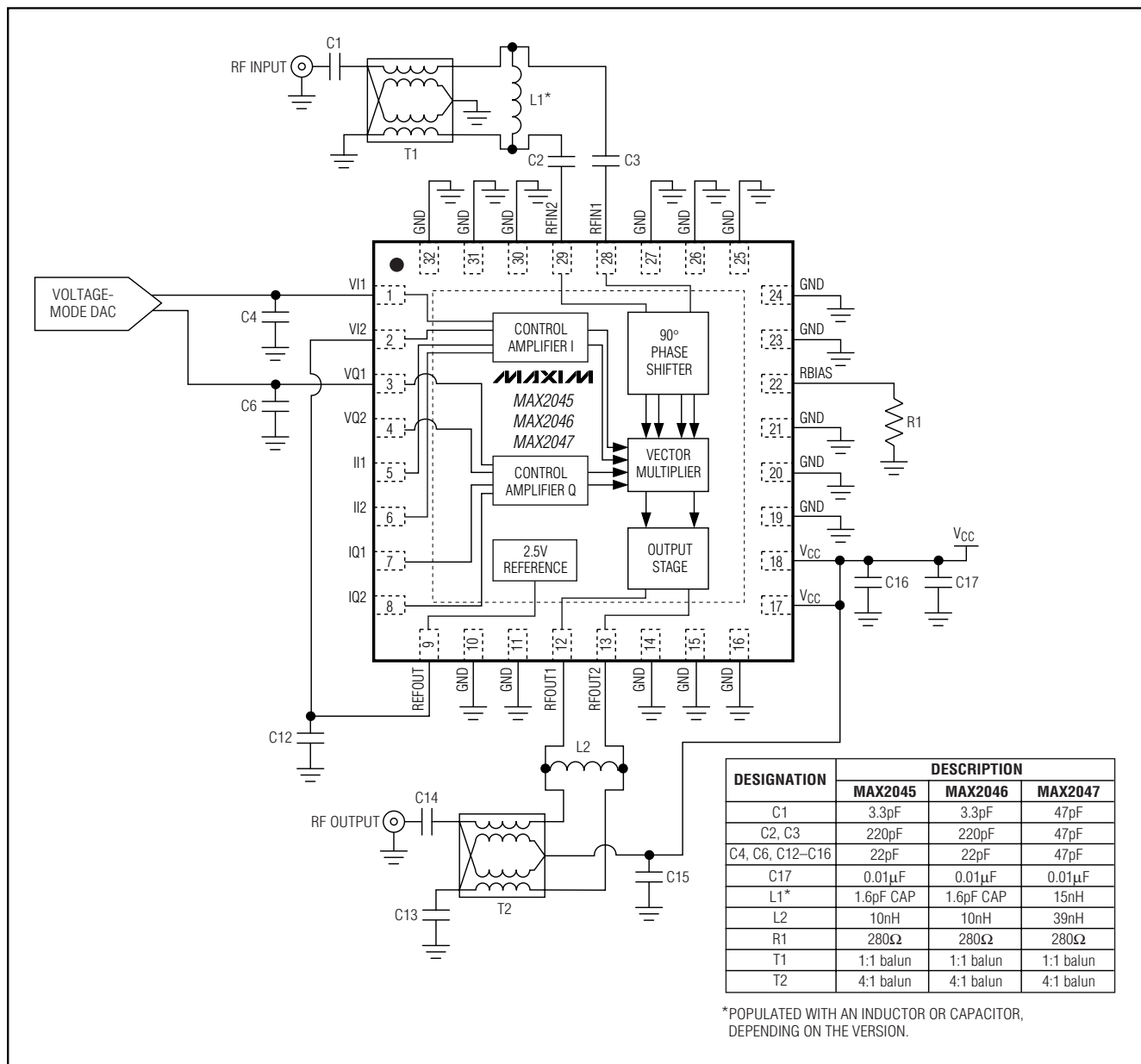
Figure 2. Typical Operating Circuit Using Single-Ended Voltage Mode DACs
