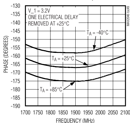
S21 PHASE vs. FREQUENCY
