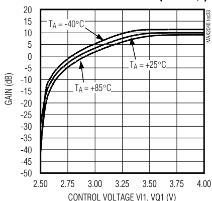
GAIN vs. CONTROL VOLTAGE (VI1 = VQ1)
